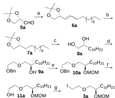
Scheme 1. a) C_8H_{17}CH=PPh_3 , 90%; b) H_2 , EtOH, Pd-C, 95%; c) HCl, MeOH; d) 1) Bu_3SnO , CHCl_3 :MeOH (10:1), reflux, 2) CsF , ICH_2CH_2OBn , DMF, 80% over 2 steps; e) MOMCl, iPr_2NH , CH_2Cl_2 , 96%; f) H_2 , EtOH, Pd-C, 90%; g) I_2 , imidazole, PPh_3 , 82%. Bn = benzyl, MOM = methoxymethyl.
